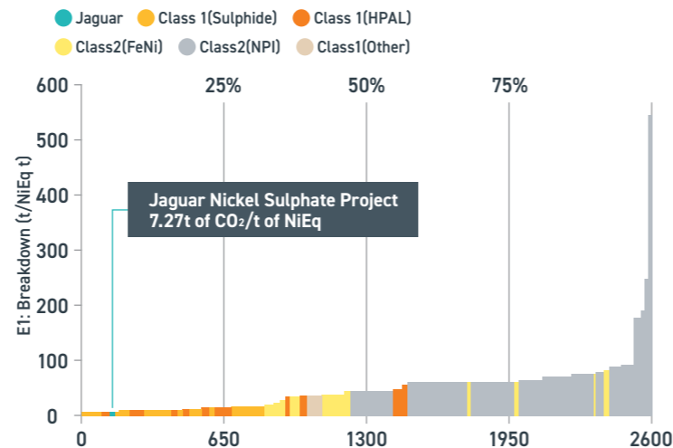
Figure 3: GHG Intensity Curve - Nickel (E1 GHG Emission Metrics ® )
